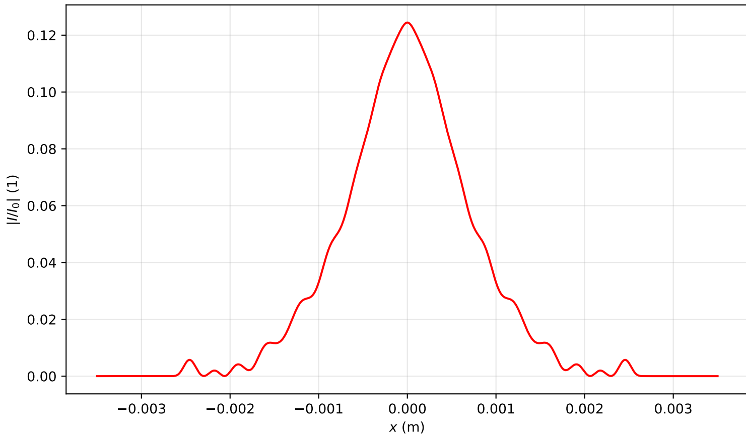
Intensity profile I(x, y = 0, z = 2.229)/I_0 , P_{in}=2.0P_{cr} , artificial time
